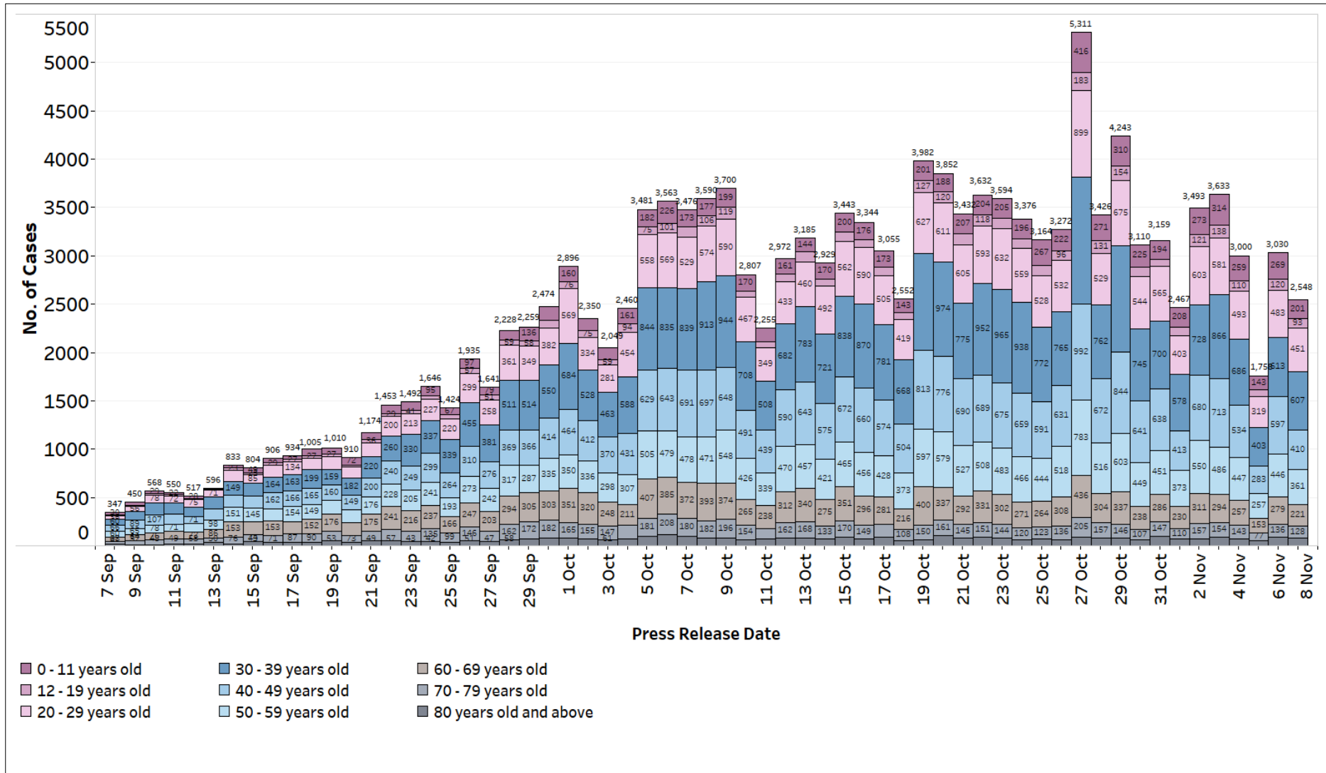
Figure 1: Number of Local Cases by Age (8 Sep – 7 Nov)
