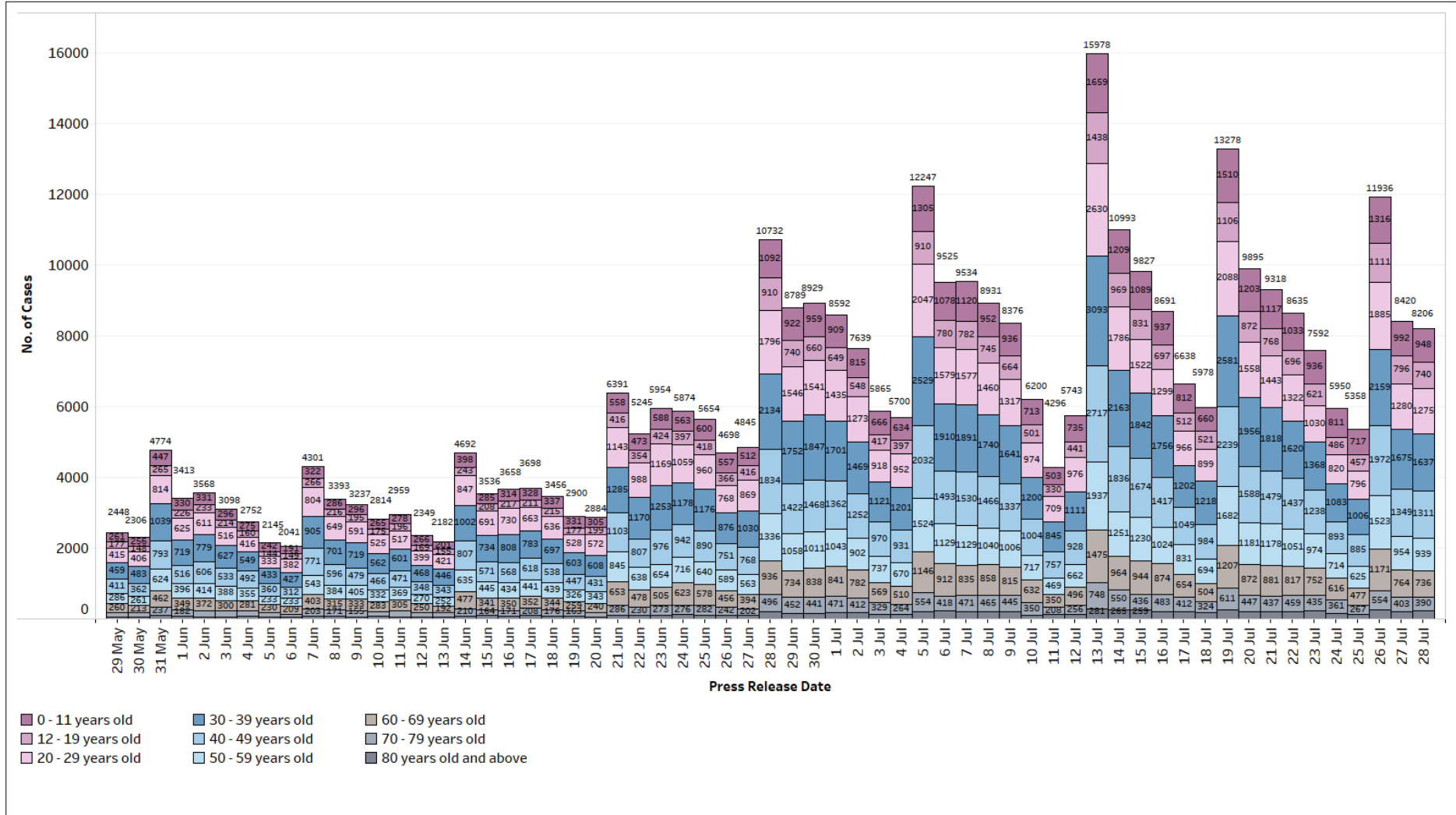
Figure 1: Number of Local PCR+ and ART+ Cases by Age (29 May – 28 Jul)
