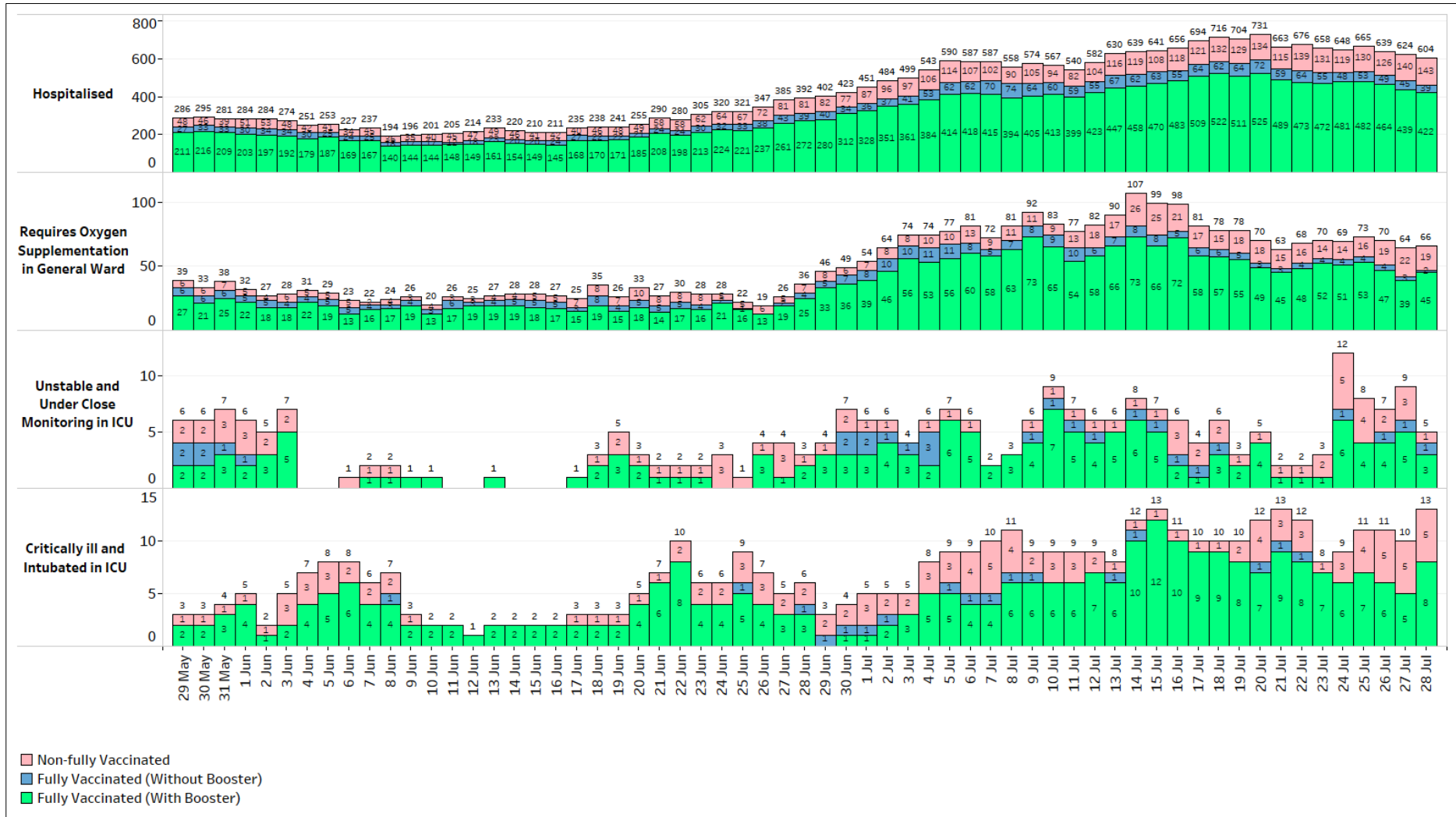
Figure 2: Active PCR+ and ART+ Cases in ICU, Requiring Oxygen Supplementation or Hospitalised 1 (29 May – 28 Jul)
