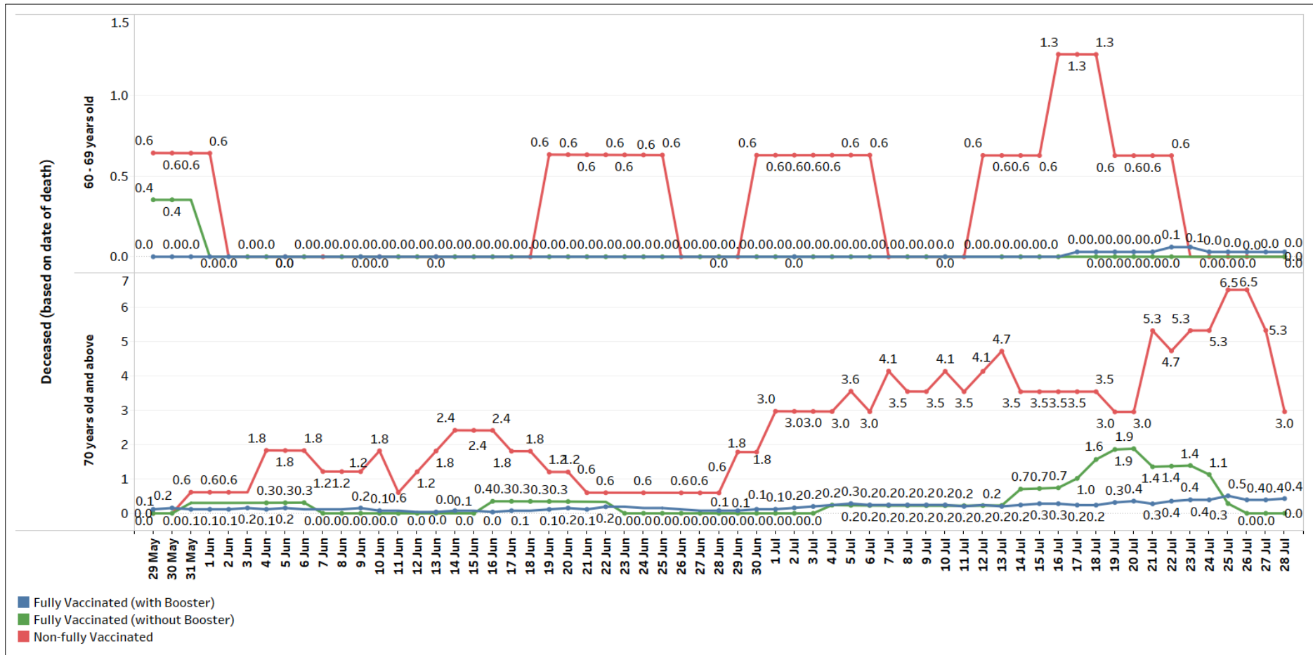
Figure 4: 7-Day Moving Average of Number of Deaths Among PCR+ and ART+ Cases between 60 – 69, and 70 years old and Above, per 100,000 Population by Vaccination Status (29 May – 28 Jul)
