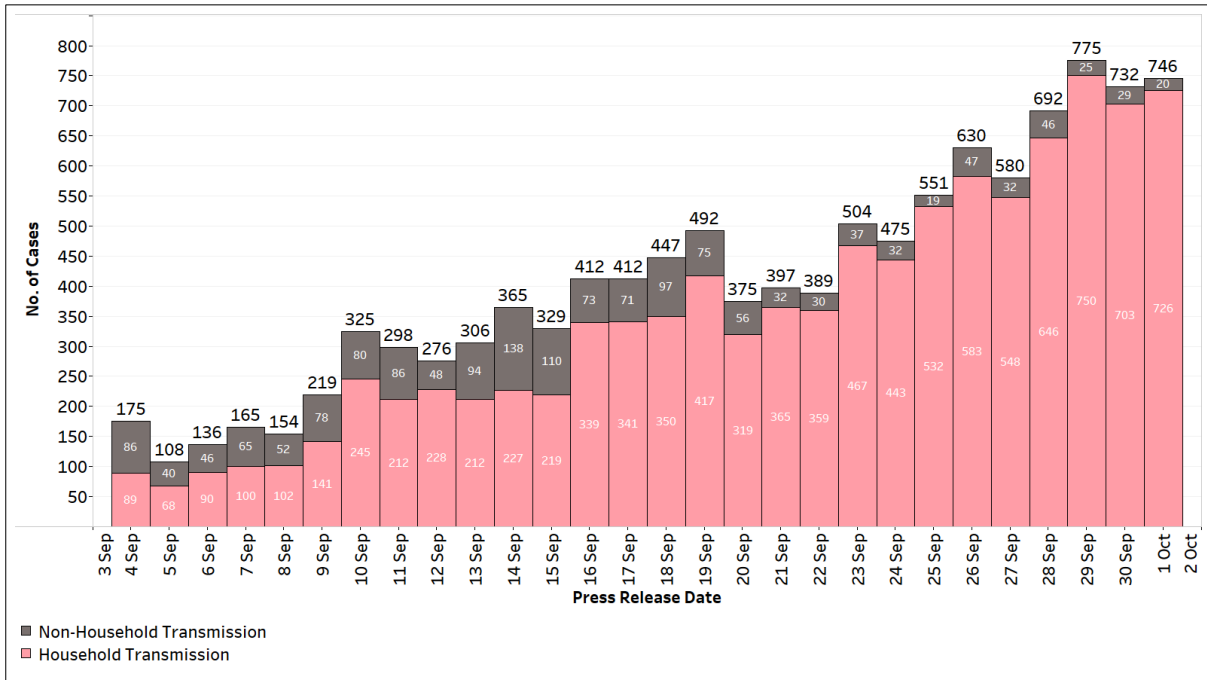
Figure 2: Number of Local Linked Cases by Household/ Non-Household Transmission 1 (4 Sep – 1 Oct)
