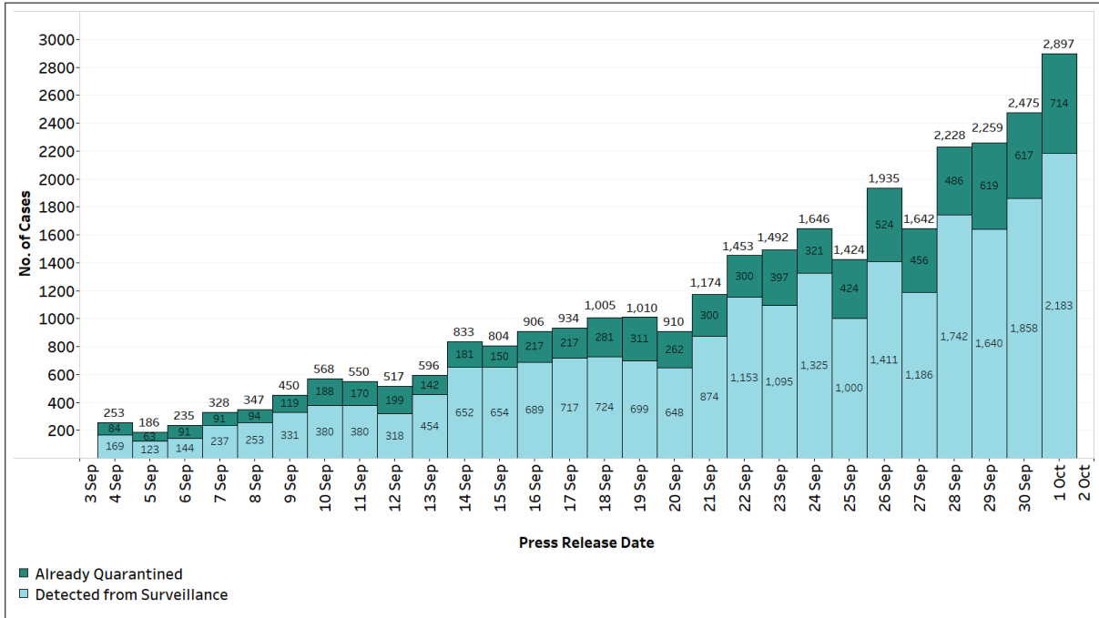
Figure 1: Number of Local Cases by Already Quarantined/ Detected from Surveillance 1 (4 Sep – 1 Oct)
