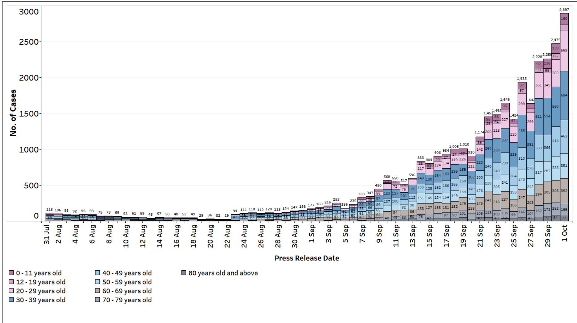
Figure 3: Number of Local Cases by Age 1 Jul – 1 Oct
