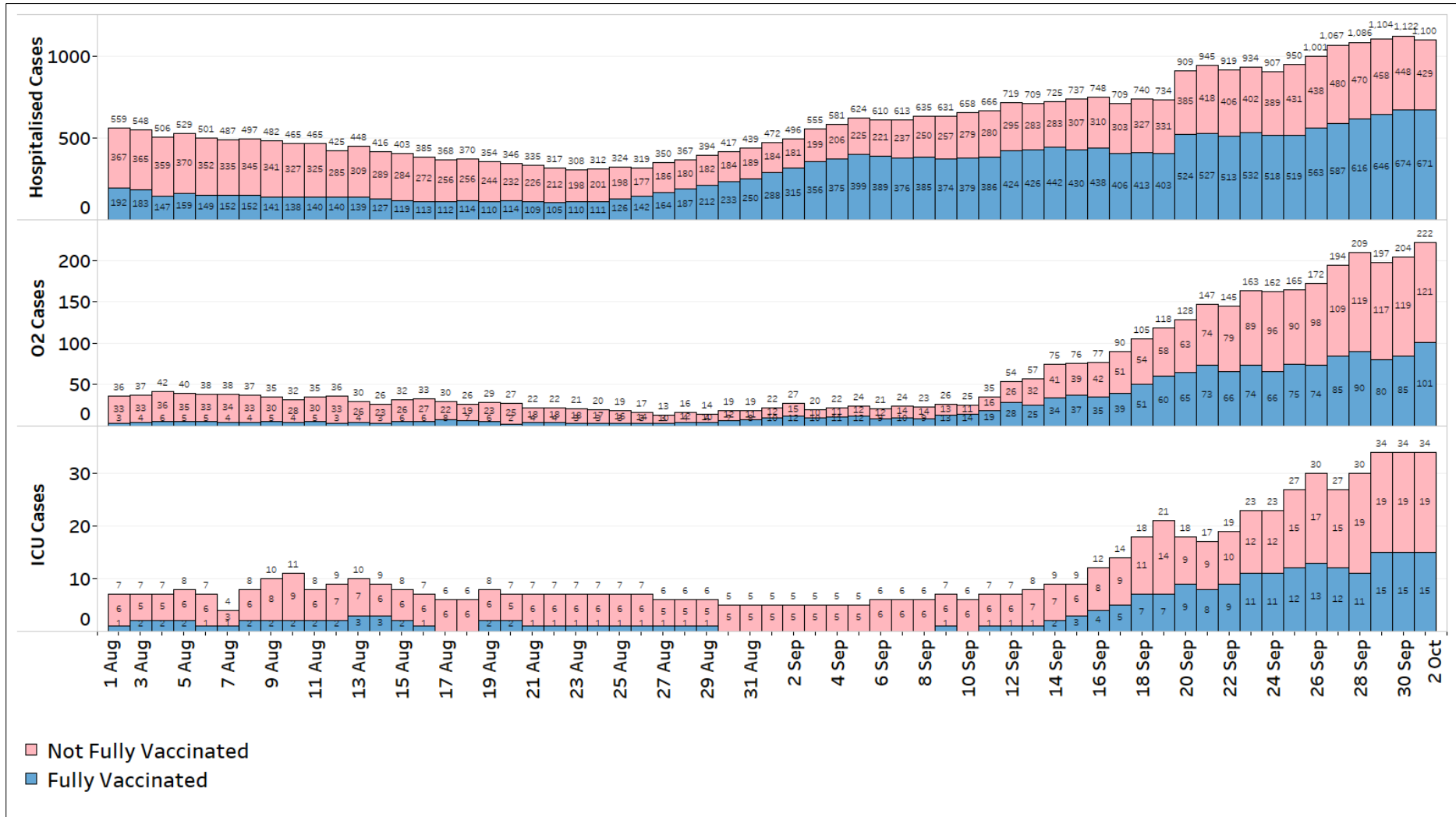
Figure 4: Active Cases in ICU, Requiring Oxygen Supplementation or Hospitalised 2 (1 Aug – 2 Oct)
