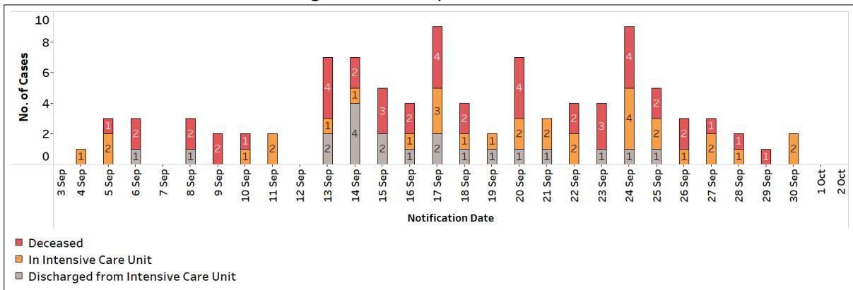
Figure 6: Deaths, Admissions into ICU and Discharges from ICU Among Local Cases by Notification Date
