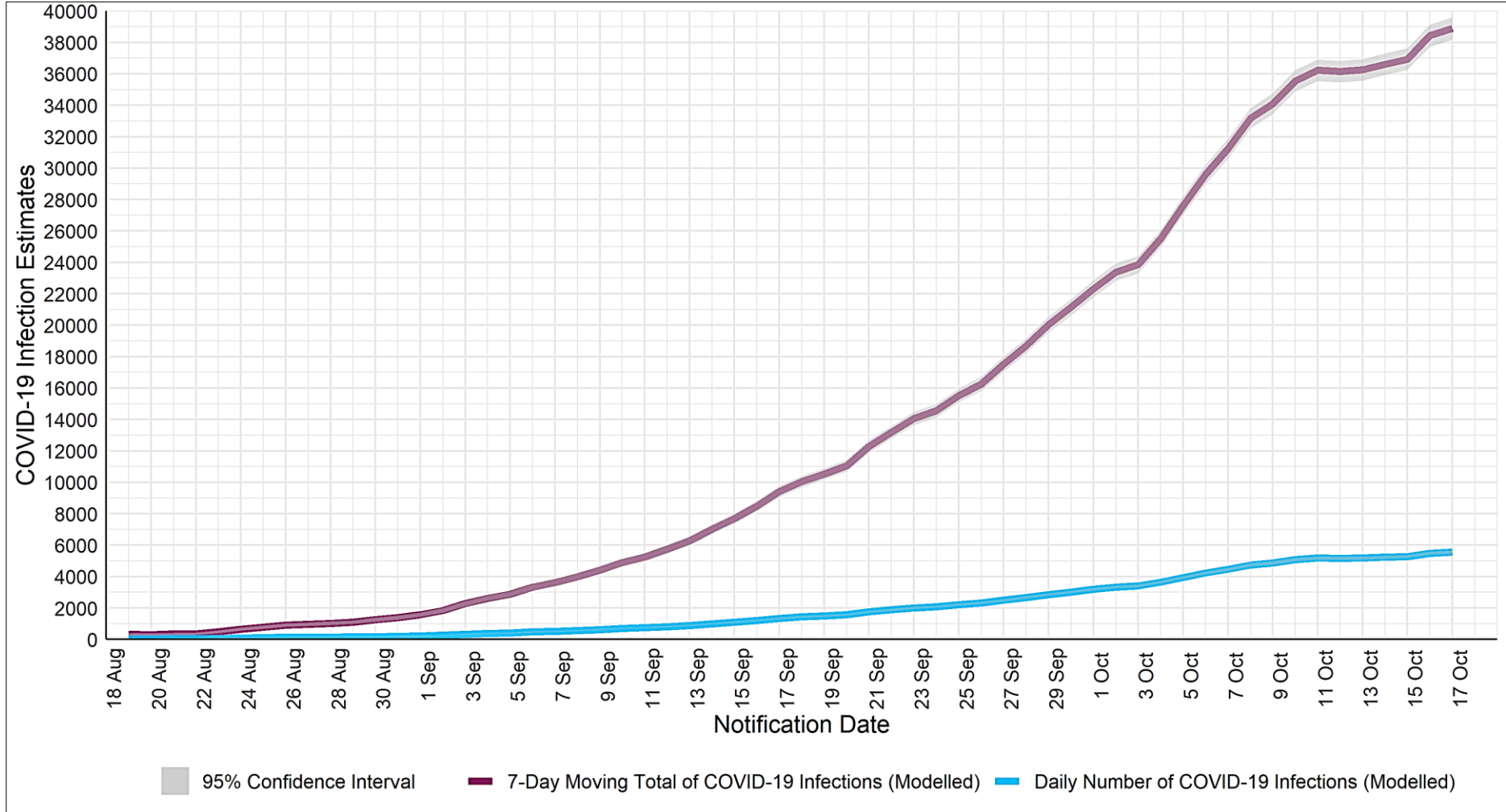
Figure 1: Modelled Number of COVID-19 Infections, Daily and 7-Day Moving Total
