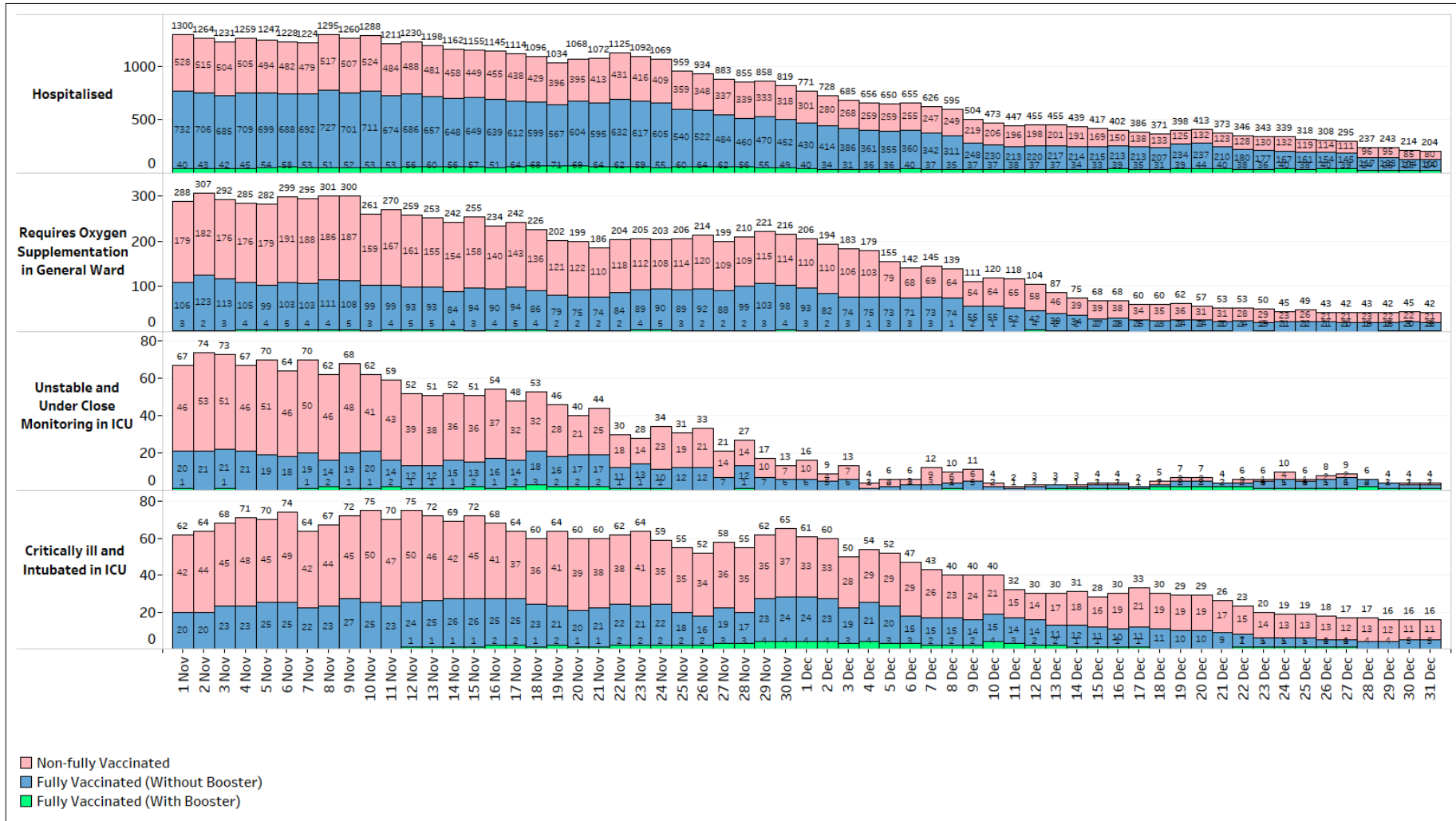
Figure 2: Active Cases in ICU, Requiring Oxygen Supplementation or Hospitalised 1 (1 Nov – 31 Dec)
