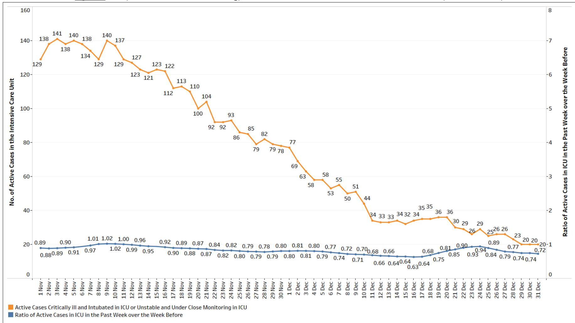
Figure 6: ICU (Intubated + Close Monitoring), Number of Cases and Week-on-Week Ratio of Cases (1 Nov – 31 Dec)
