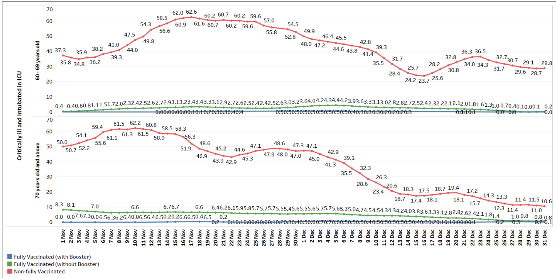
Figure 3: 7-Day Moving Average of Number of Active Cases between 60 – 69, and 70 years old and Above that are Critically ill and Intubated in ICU, per 100,000 Population by Vaccination Status (1 Nov – 31 Dec)
