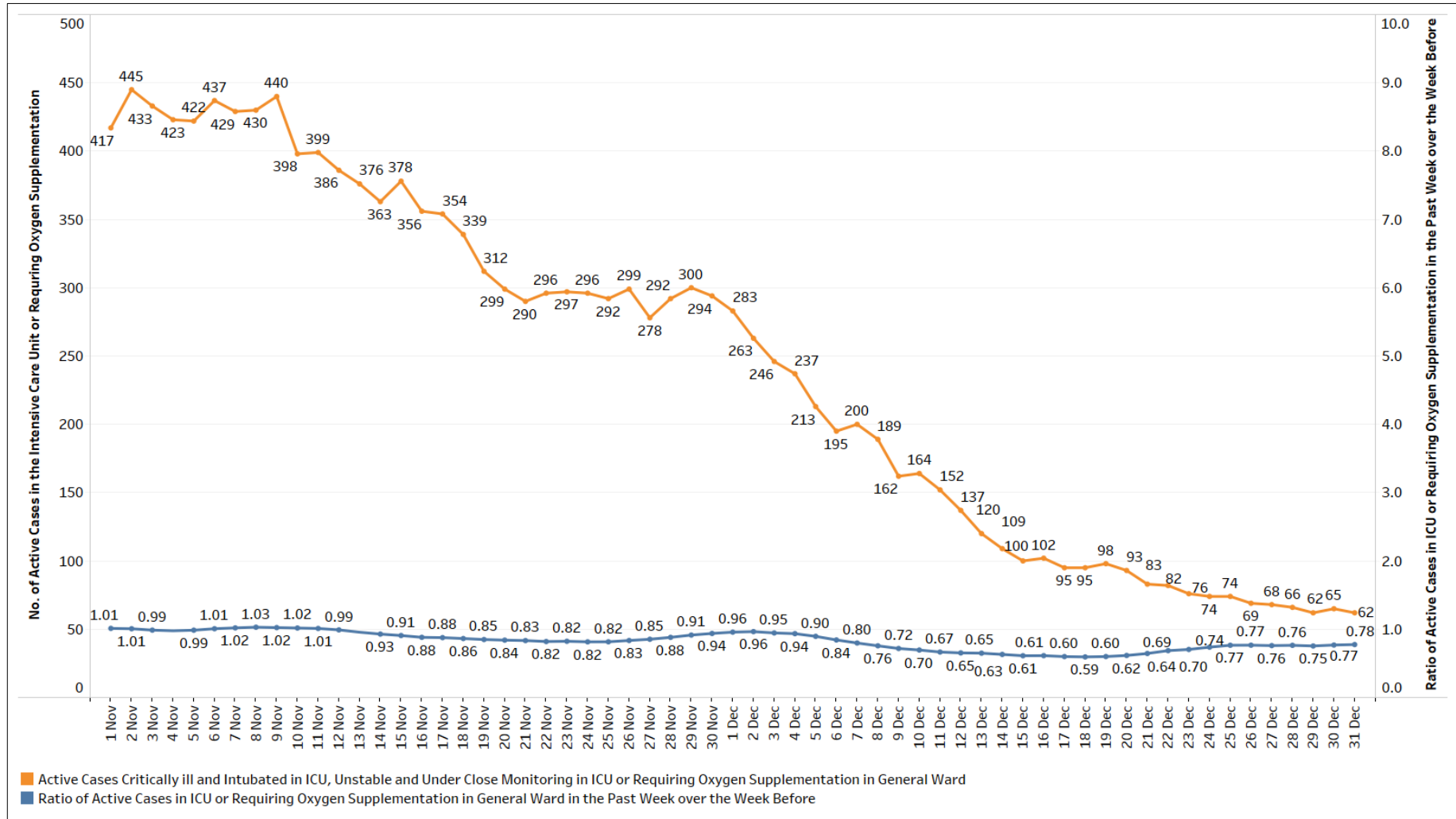
Figure 5: General Wards O2 + ICU (Intubated + Close Monitoring), Number of Cases and Week-on-Week Ratio of Cases (1 Nov – 31 Dec)
