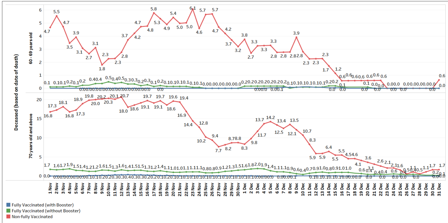
Figure 4: 7-Day Moving Average of Number of Deaths between 60 – 69, and 70 years old and Above, per 100,000 Population by Vaccination Status (1 Nov – 31 Dec)
