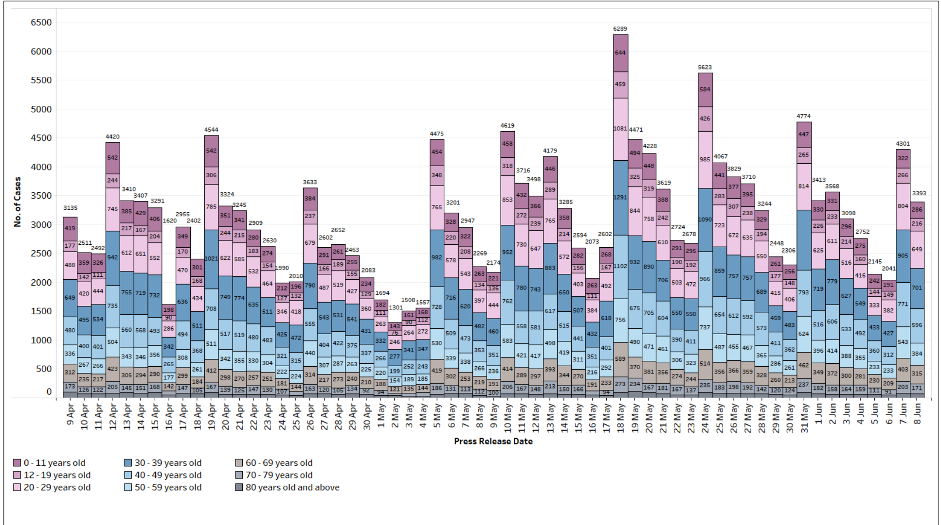
Figure 1: Number of Local PCR+ and ART+ Cases by Age (9 Apr – 8 Jun)
