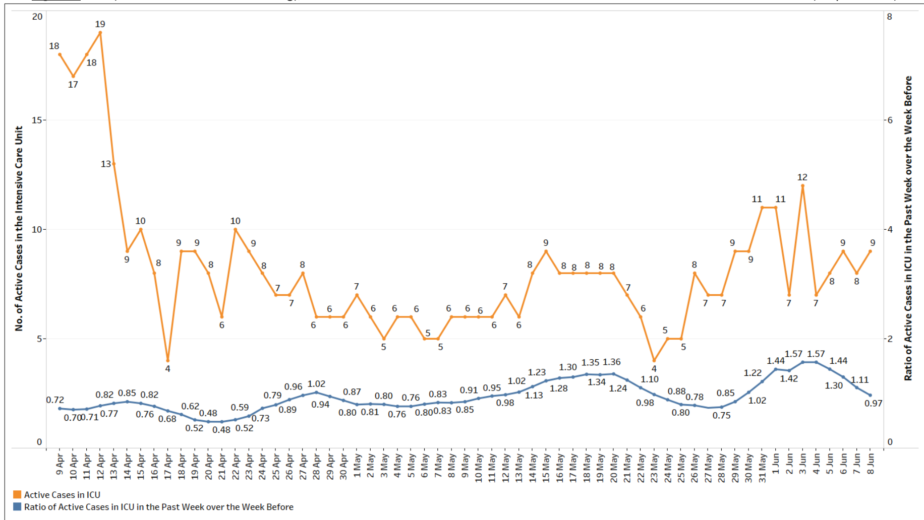
Figure 6: ICU (Intubated + Close Monitoring), Number of PCR+ and ART+ Cases and Week-on-Week Ratio of PCR+ and ART+ Cases (9 Apr – 8 Jun)
