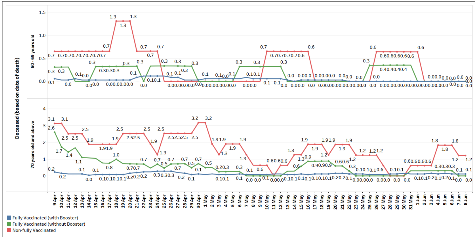
Figure 4: 7-Day Moving Average of Number of Deaths Among PCR+ and ART+ Cases between 60 – 69, and 70 years old and Above, per 100,000 Population by Vaccination Status (9 Apr – 8 Jun)
