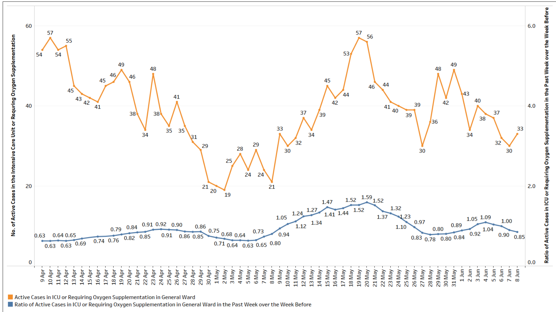
Figure 5: General Wards O2 + ICU (Intubated + Close Monitoring), Number of PCR+ and ART+ Cases and Week-on-Week Ratio of PCR+ and ART+ Cases (9 Apr – 8 Jun)
