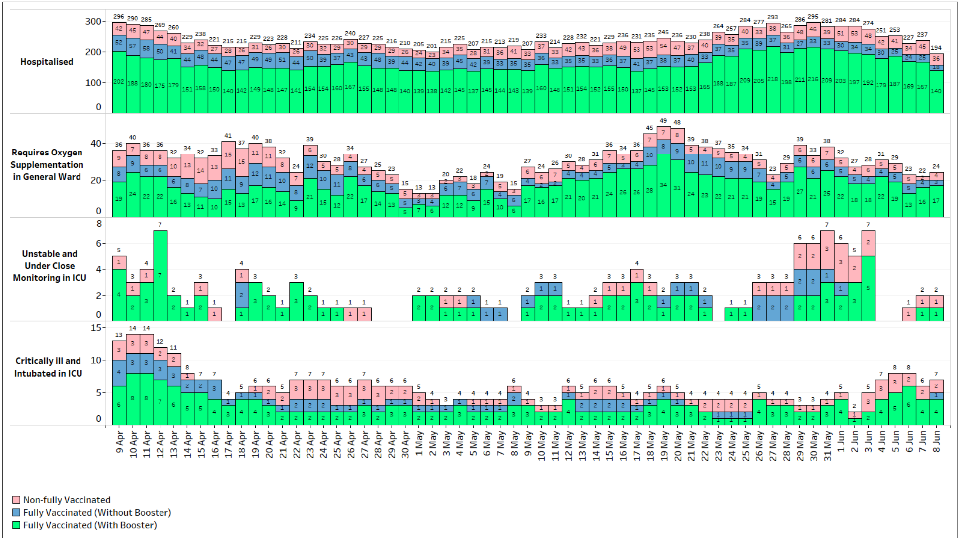
Figure 2: Active PCR+ and ART+ Cases in ICU, Requiring Oxygen Supplementation or Hospitalised 1 (9 Apr – 8 Jun)
