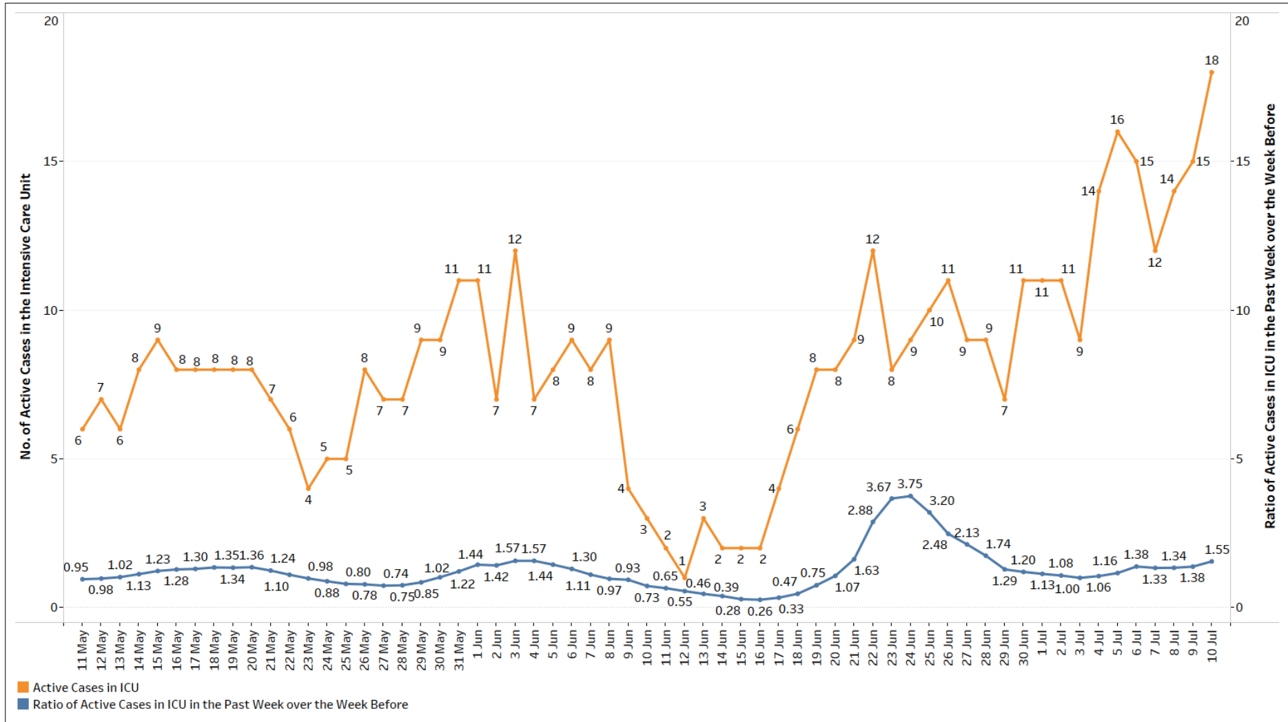
Figure 6: ICU (Intubated + Close Monitoring), Number of PCR+ and ART+ Cases and Week-on-Week Ratio of PCR+ and ART+ Cases (11 May – 10 Jul)
