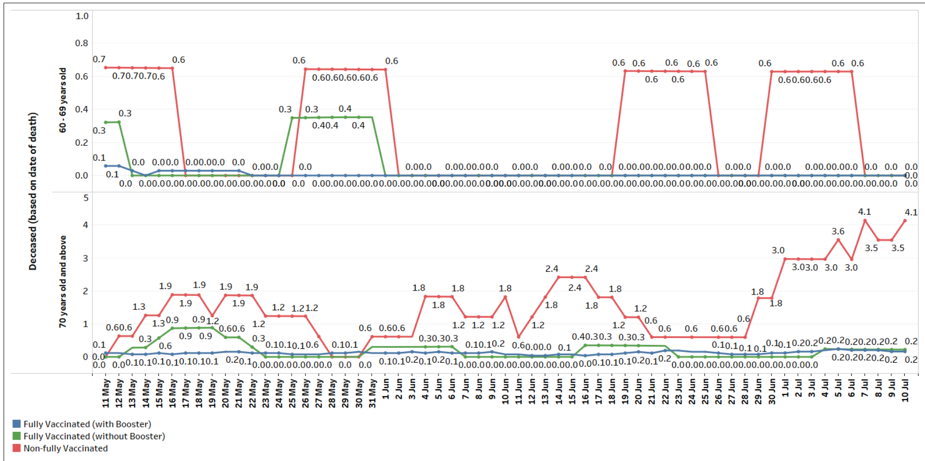
Figure 4: 7-Day Moving Average of Number of Deaths Among PCR+ and ART+ Cases between 60 – 69, and 70 years old and Above, per 100,000 Population by Vaccination Status (11 May – 10 Jul)
