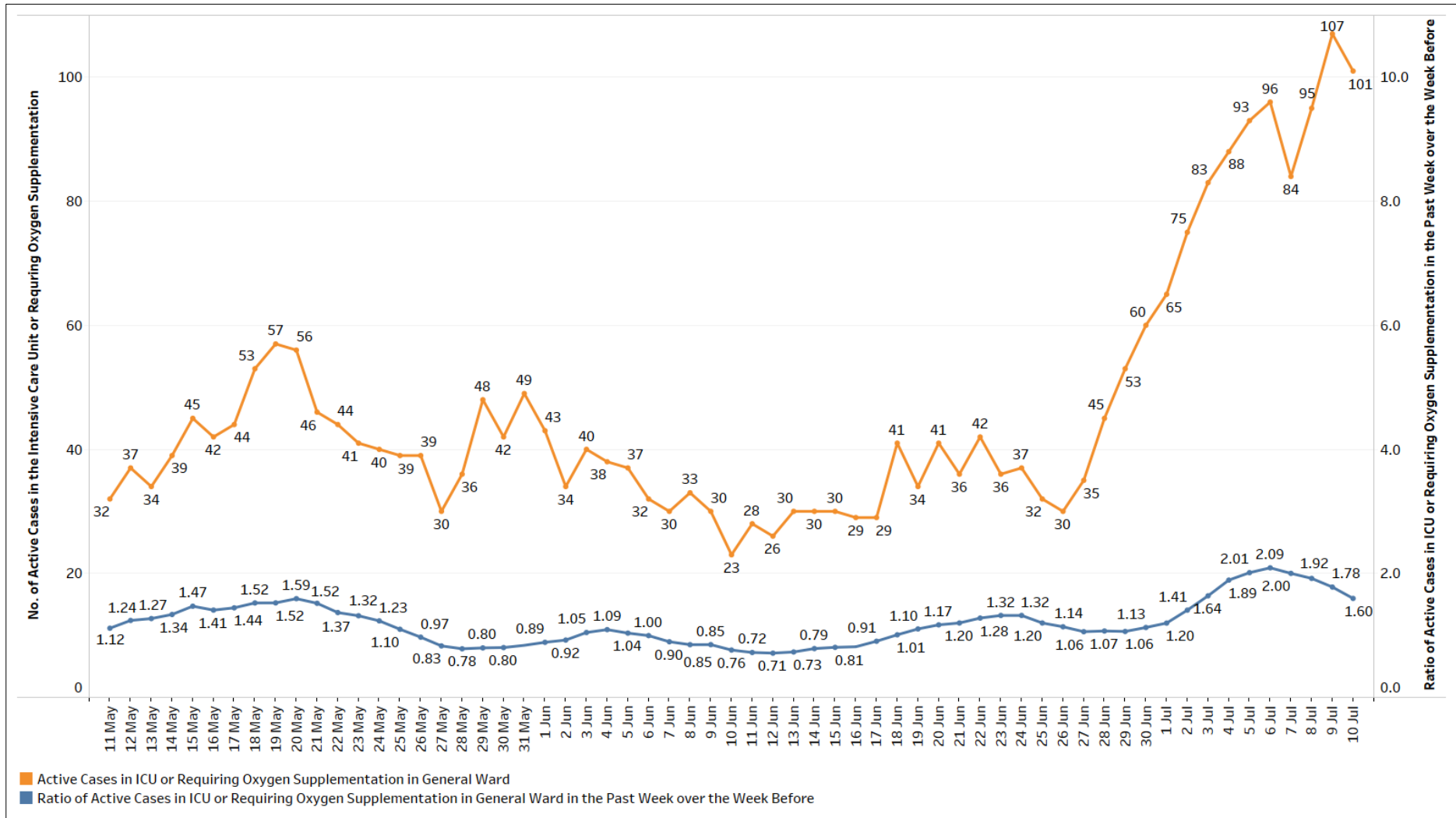
Figure 5: General Wards O2 + ICU (Intubated + Close Monitoring), Number of PCR+ and ART+ Cases and Week-on-Week Ratio of PCR+ and ART+ Cases (11 May – 10 Jul)
